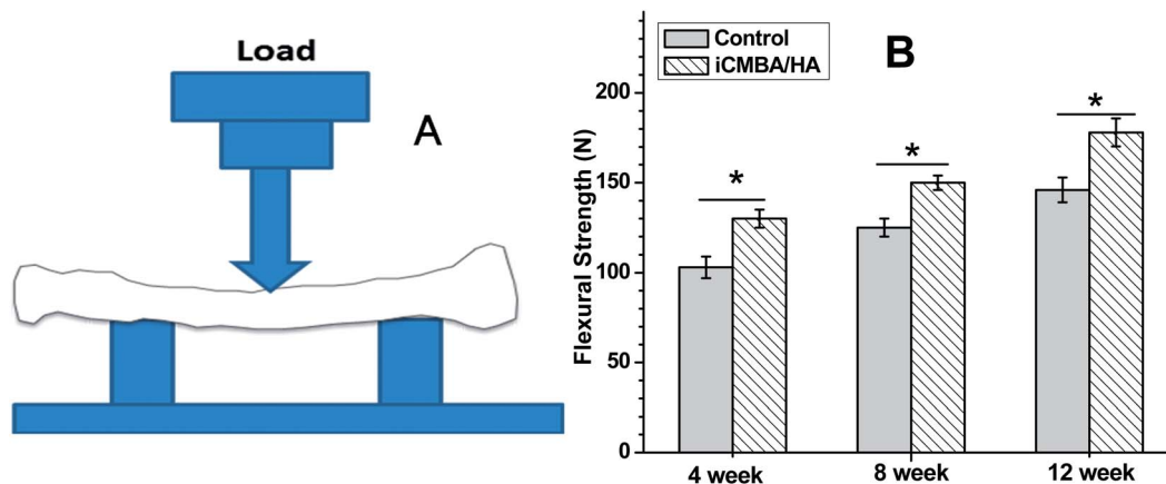
Fig. 12 Three-point-bending test was performed of on MTS machine for comminuted fracture area of radius bone. Maximal flexural strength was recorded. *: significant difference ( p < 0.05 ).
