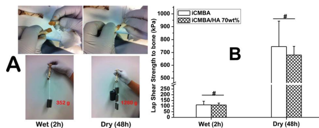
Fig. 4 (A) Application of iCMBA/HA 70 wt% (8 wt% PI) to beveled (beveling angle: 30^\circ ) chicken bone (top) and the strong adhesion demonstrated by hanging metal pieces (low); (B) wet (2 h) and dry (48 h) adhesion strengths of iCMBA (iCMBA- P_{200} D_{0.3} , 40 wt% in DI water) and iCMBA/HA 70 wt% to chicken bones after applying equal volume of 8 wt% PI [Sodium (meta) periodate, NaIO_4 ] solution. # represents p > 0.05 .
